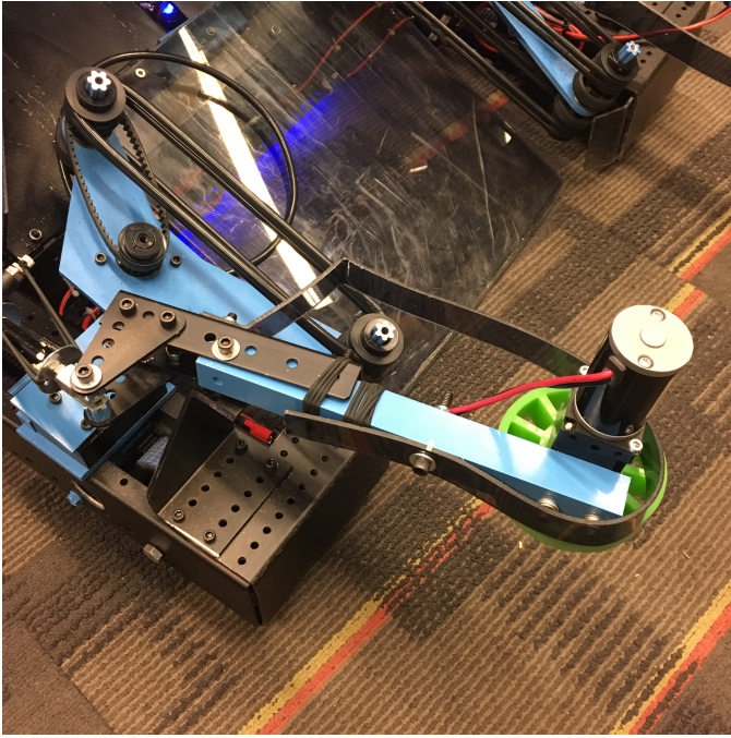
Fig. 4. A look at the elastic joint– the blue bar pivots around the bolt attaching it to the black part
