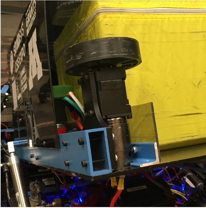
Fig. 10. The VersaPlanetarys were mounted to the shooter using custom waterjetted 1/4" aluminum plates
