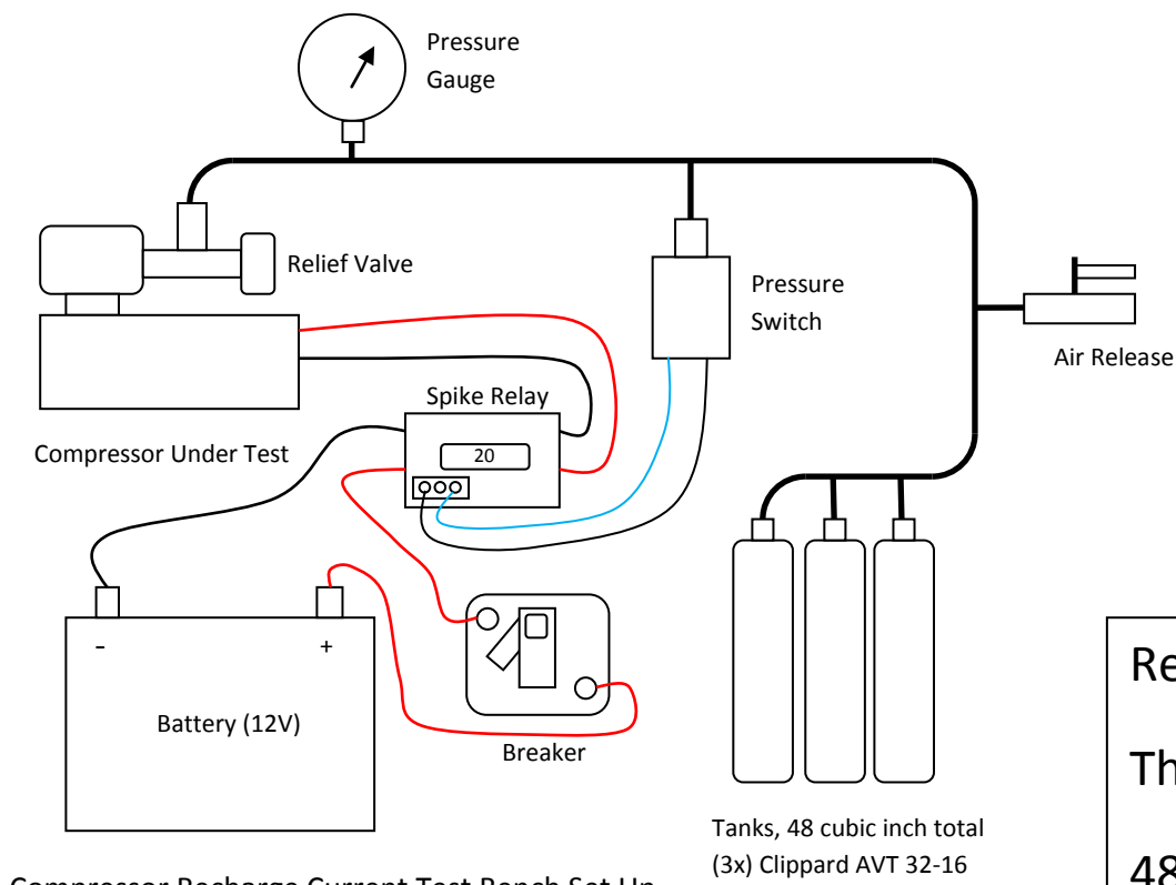
Compressor Recharge Current Test Bench Set Up
