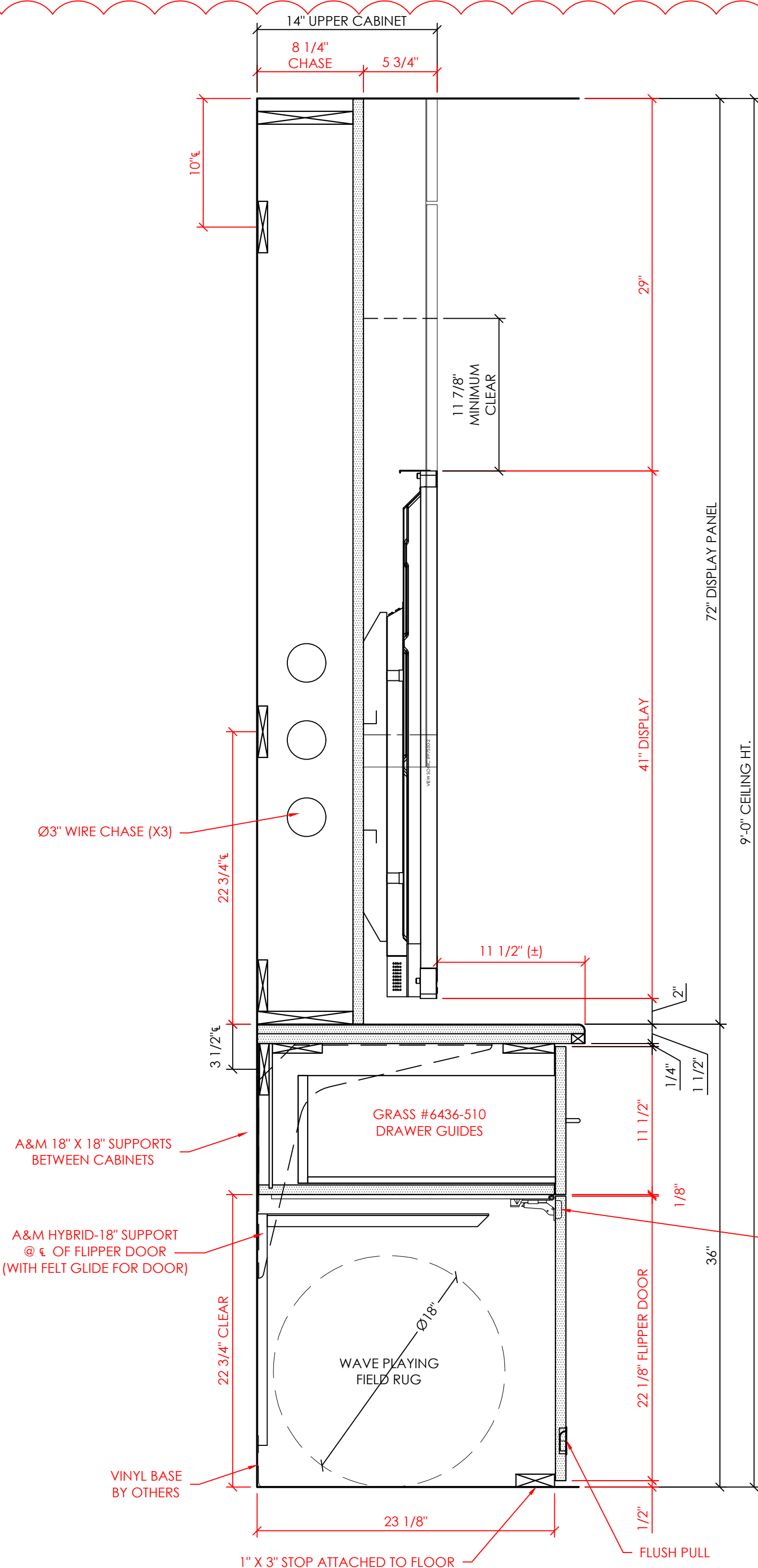
3.1 DETAIL SCALE: 1 1/2" = 1'-0" ARCH. REF.: - / -
