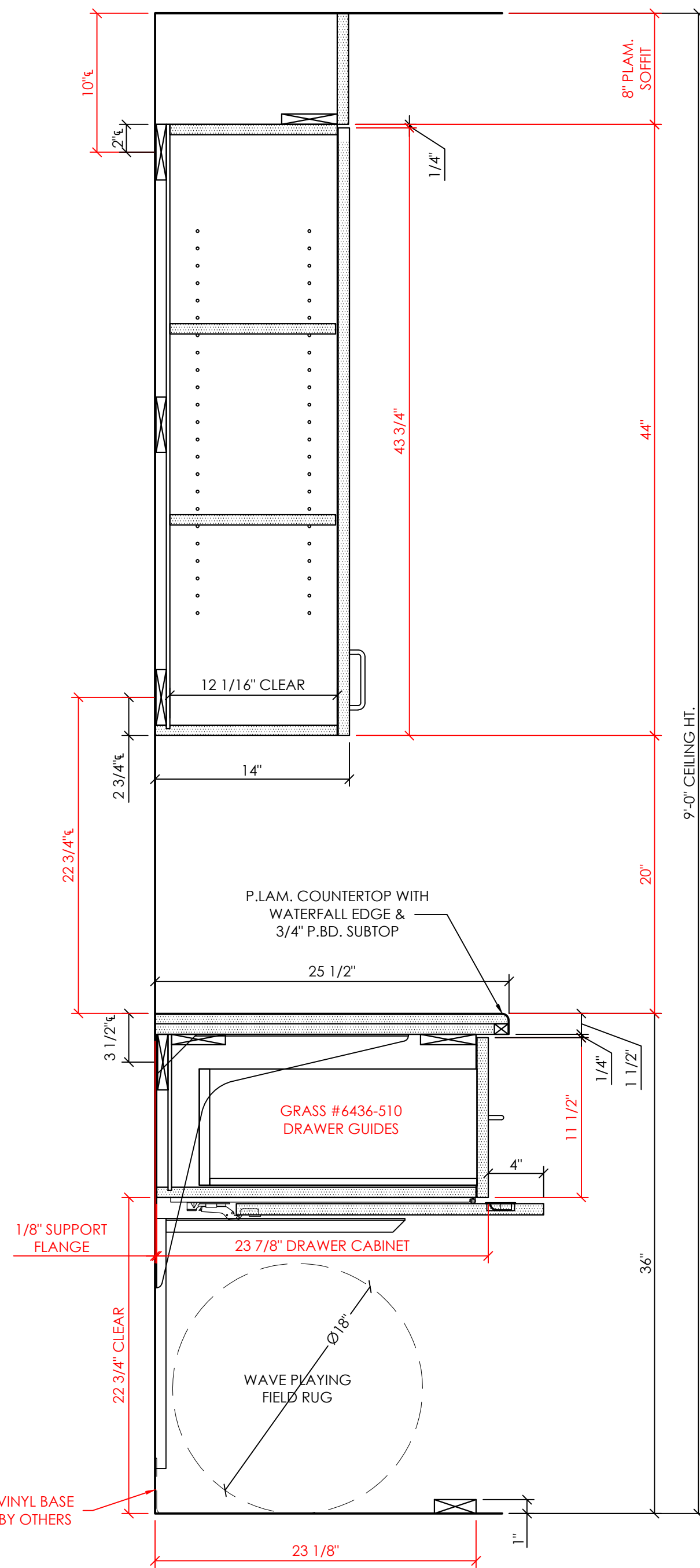
3.1 DETAIL SCALE: 1 1/2" = 1'-0" ARCH. REF.: - / -
