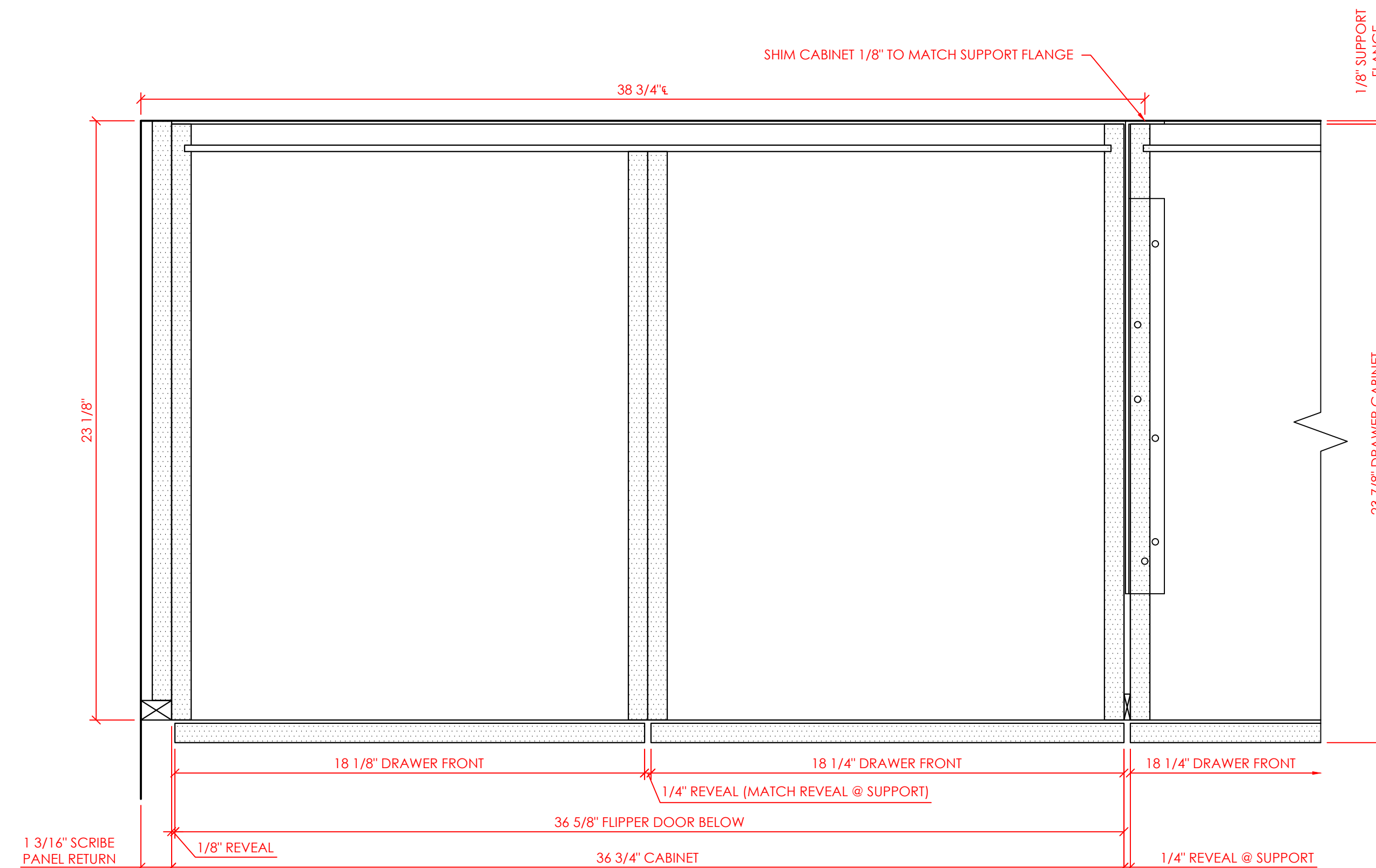
7.1 DETAIL SCALE: 3" = 1'-0" ARCH. REF.: - / -
