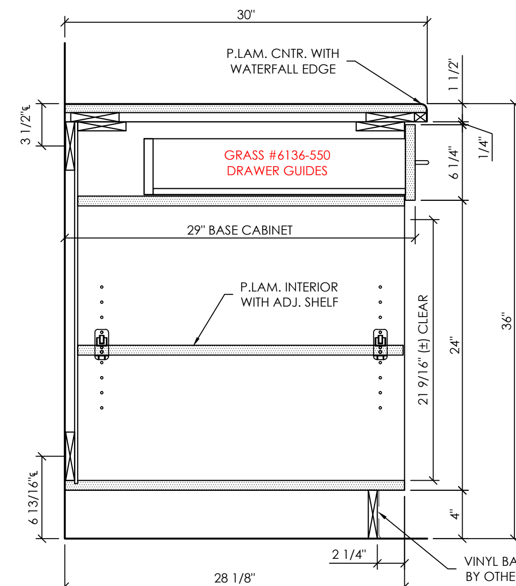
3.1 DETAIL SCALE: 1 1/2" = 1'-0" ARCH. REF.: - / -
