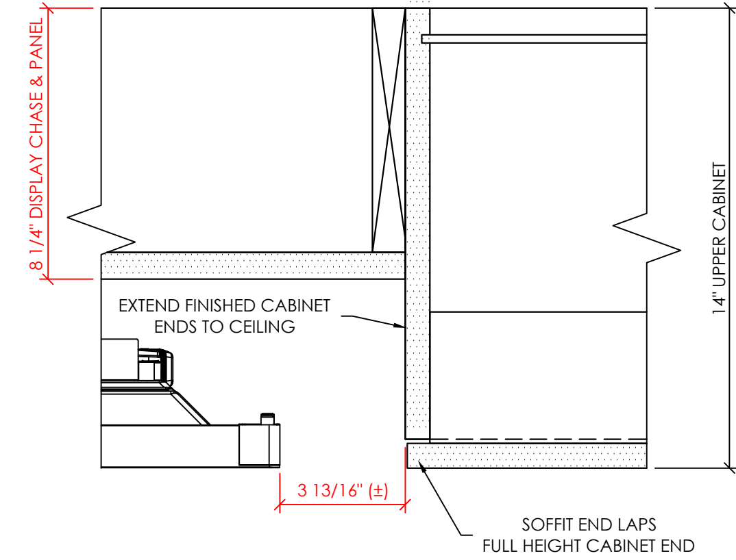
5.1 DETAIL SCALE: 3" = 1'-0" ARCH. REF.: - / -
